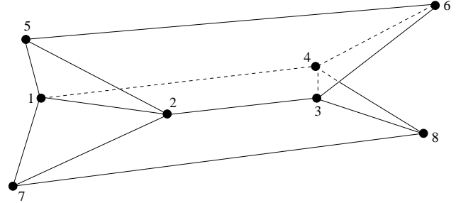
Fig. 1. A geometric description of the Vámos matroid.
