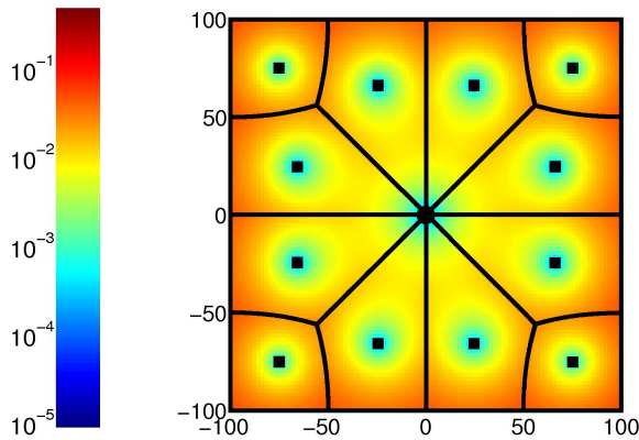
Fig. 1. Algorithm and simulation output for amplify-and-forward over fading channels with N = 12 , G = 75 dB, and E_{R_x}/N_0|_{d=50\text{ m}} = 5 dB. Relays are denoted by black squares and the receiver is located at (0, 0) . Sensors are distributed as a square grid over \pm 100 meters in each dimension. The optimal sensor regions \sigma_1, \dots, \sigma_{12} are separated by black boundaries.
