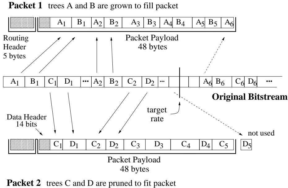
Figure 1: The encoder decides to put trees A and B into packet 1, and trees C and D into packet 2. Because trees A and B do not quite fill the packet, they are grown by using additional bits from beyond the target rate. Trees C and D together overflow their packet, and so get pruned.
