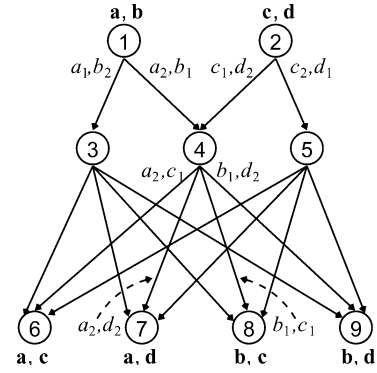
Fig. 5. The network \mathcal{N}_6 whose routing capacity is 1.
