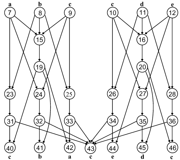
Fig. 7. The network \mathcal{N}_8 whose routing capacity is 1/3 .
