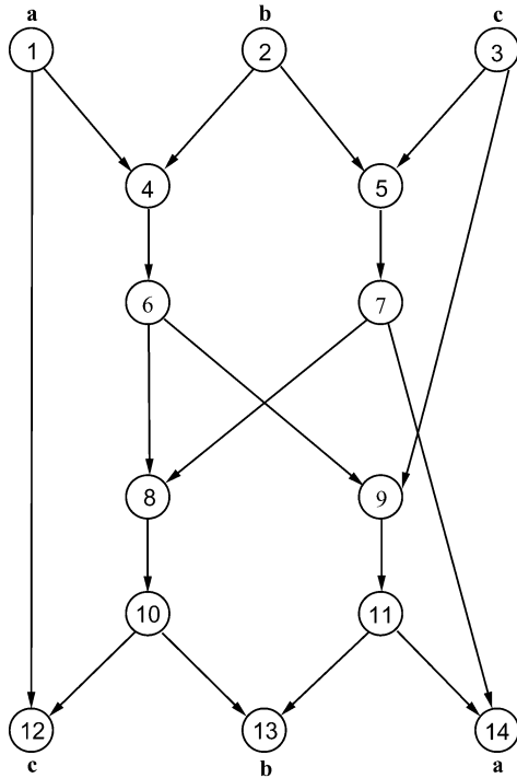
Fig. 6. The network \mathcal{N}_7 whose routing capacity is 2/3 .
