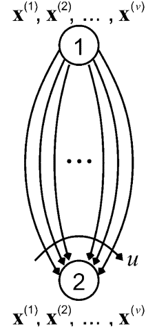
Fig. 10. A network \mathcal{N}_9 that has routing capacity r = u/v \geq 0 .
