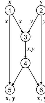
Fig. 2. The network \mathcal{N}_2 whose routing capacity is 1/2 .
