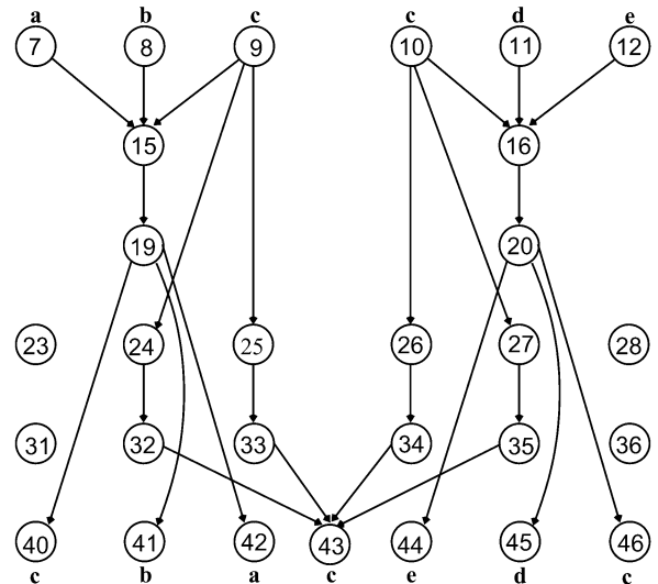
Fig. 8. Reduced form of the network \mathcal{N}_8 given in Fig. 7.
